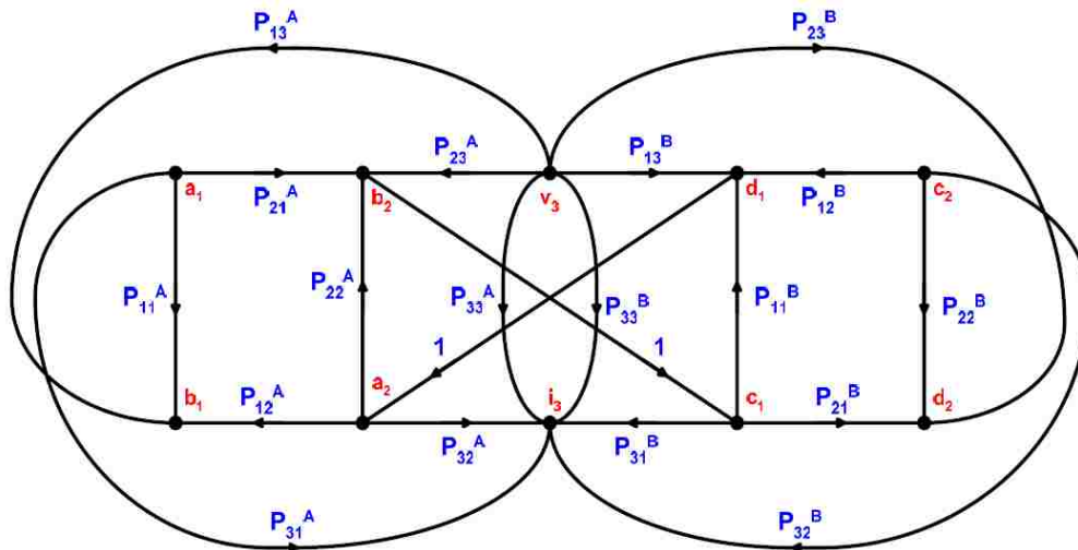
Figure B-3. Signal flow graph for P-Matrix cascade with parallel electrical connection. Image of D. Puccio, from Figure 4-6 of his dissertation [8]. Port 3 is the electrical port.
