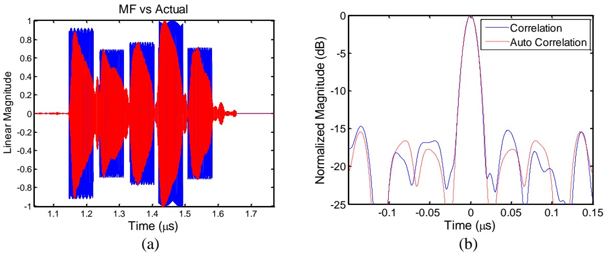
Figure 2-8. (a) Measured OFC sensor time response (red) and corresponding matched filter (blue) created from truncated cosine functions. (b) Shows that the correlation of the measured sensor response with matched filter is very close to the auto-correlation of the ideal matched filter.
