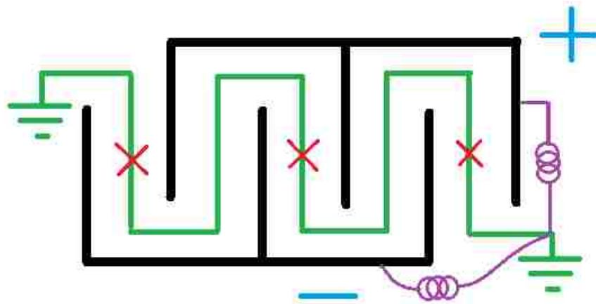
Figure B-10. Schematic of phased meander-ground GUDT. The x's correspond to the x's in Figure B-11.
