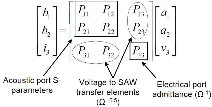
Figure B-1. The mixed P-Matrix description of 1 dimensional SAW structures with its entries grouped into like units. Image of D. Puccio, from Figure 4-4 of his dissertation [8].
