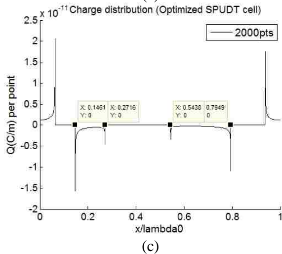
Figure E-4. The charge distribution (a) (c) and frequency domain representation of charge distribution (b) (d) for both the EWC and enhanced 3 rd harmonic SPUDT, respectively. A voltage of +/- 1/2V is placed on the electrodes in order to generate these values. —the total (+) charge of (c) is 5.06e-10C/m.
