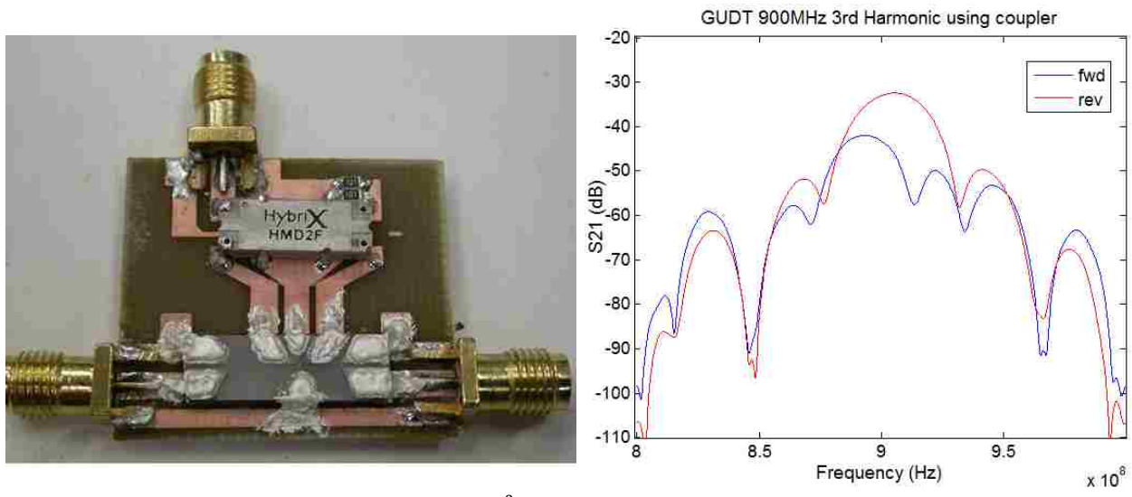
Figure A-10. Hybrid coupler used to provide the 90^{\circ} phase shift with equal power split and demonstrate the operation of the 3 rd harmonic device. Comparing the side lobe levels, it doesn't seem like an equal power split for forward and reverse direction was achieved, nor the 90^{\circ} phase shift—an imbalance in the I and Q group impedance may contribute to the skewing of the reverse response.
