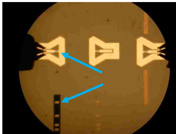
Figure 2-3. Reflective delay line device with top arrow pointing to IDT being probed. Bottom arrow is pointing to a set of reflectors covered with an SiO 2 film. The device has an identical set of uncovered reference reflectors on the other side of the IDT. The reference reflectors are set at twice the distance and are outside the field of view of the microscope but would be similar to the uncovered reflectors of the adjacent middle device.
