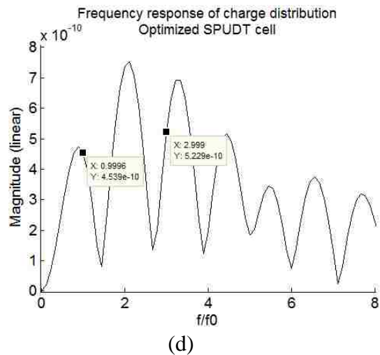
Figure E-4. The charge distribution (a) (c) and frequency domain representation of charge distribution (b) (d) for both the EWC and enhanced 3 rd harmonic SPUDT, respectively. A voltage of +/- 1/2V is placed on the electrodes in order to generate these values. —the total (+) charge of (c) is 5.06e-10C/m.
