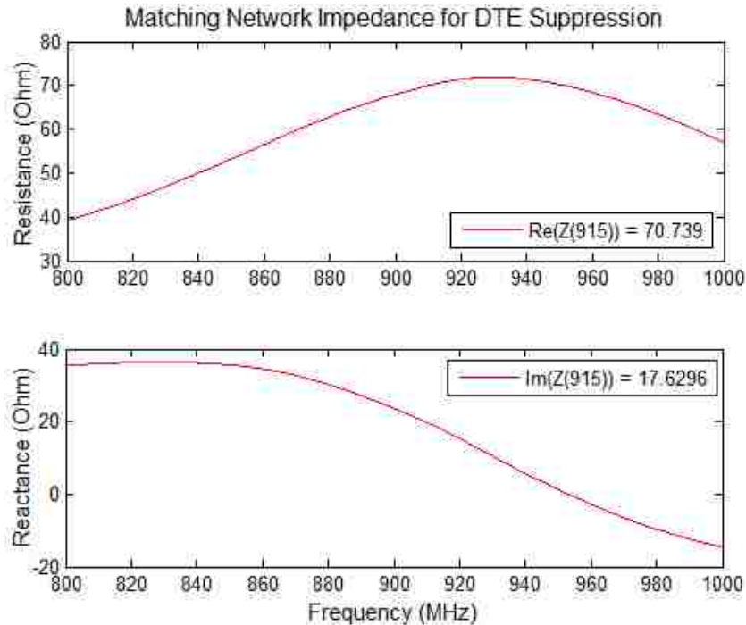
Figure 6-8. Impedance profile of the matching network as seen by the 3 rd harmonic SPUDT, tuned for optimized DTE suppression—71+j18Ohm at 915MHz, Figure 6-7a.
